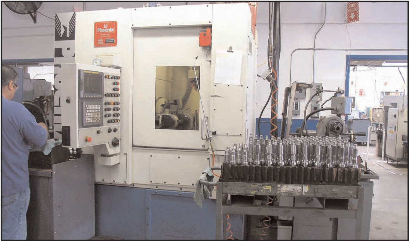
Gleason 125GH CNC Gear Hobb
