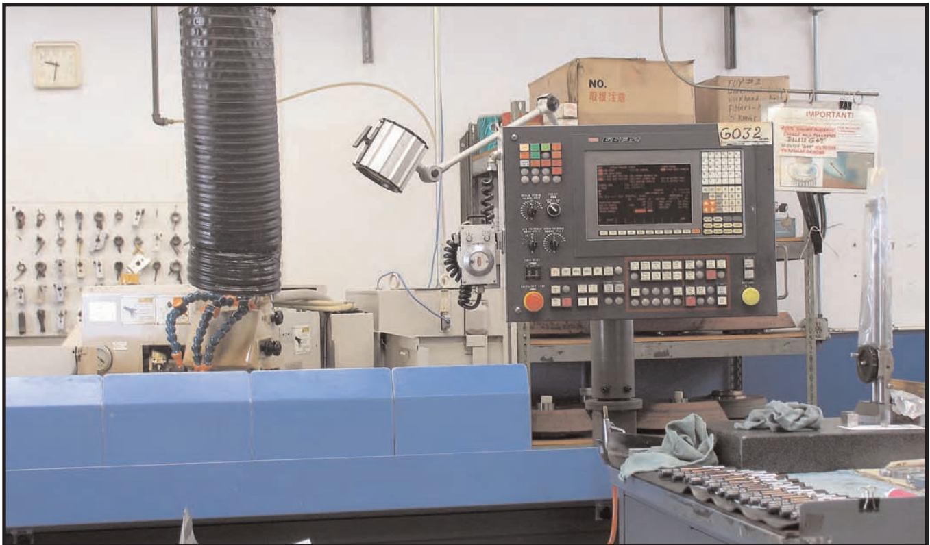
Toyoda CNC Angle Head Grinder Capacity 1000mm/39.4" between centers
