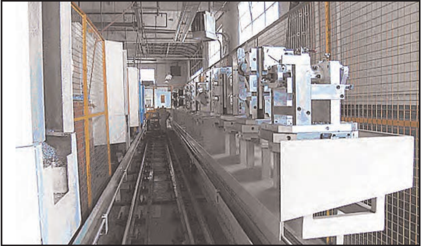
Toyota 450III 40Taper Horizontal W/200 Tool Tools
